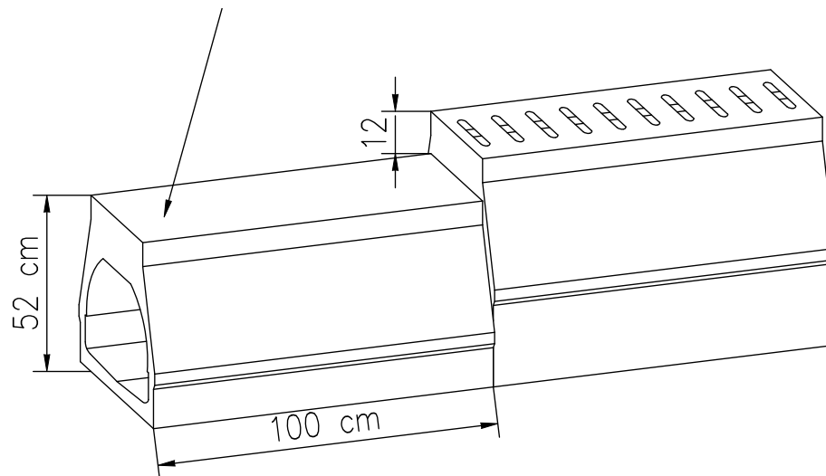
Prerez tunel brez reŝ
